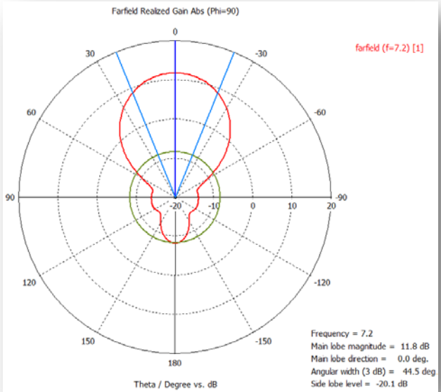
YZ Plane
