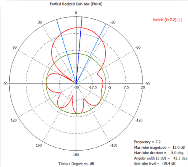
XZ Plane
